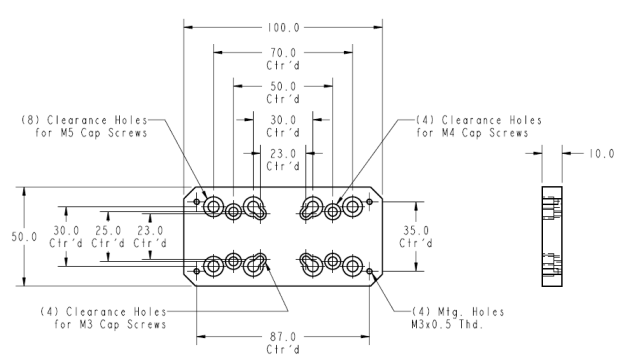
002-2825-01 Transition Plate
