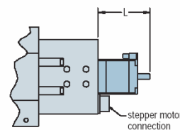
Mounting - Stepper Motor
