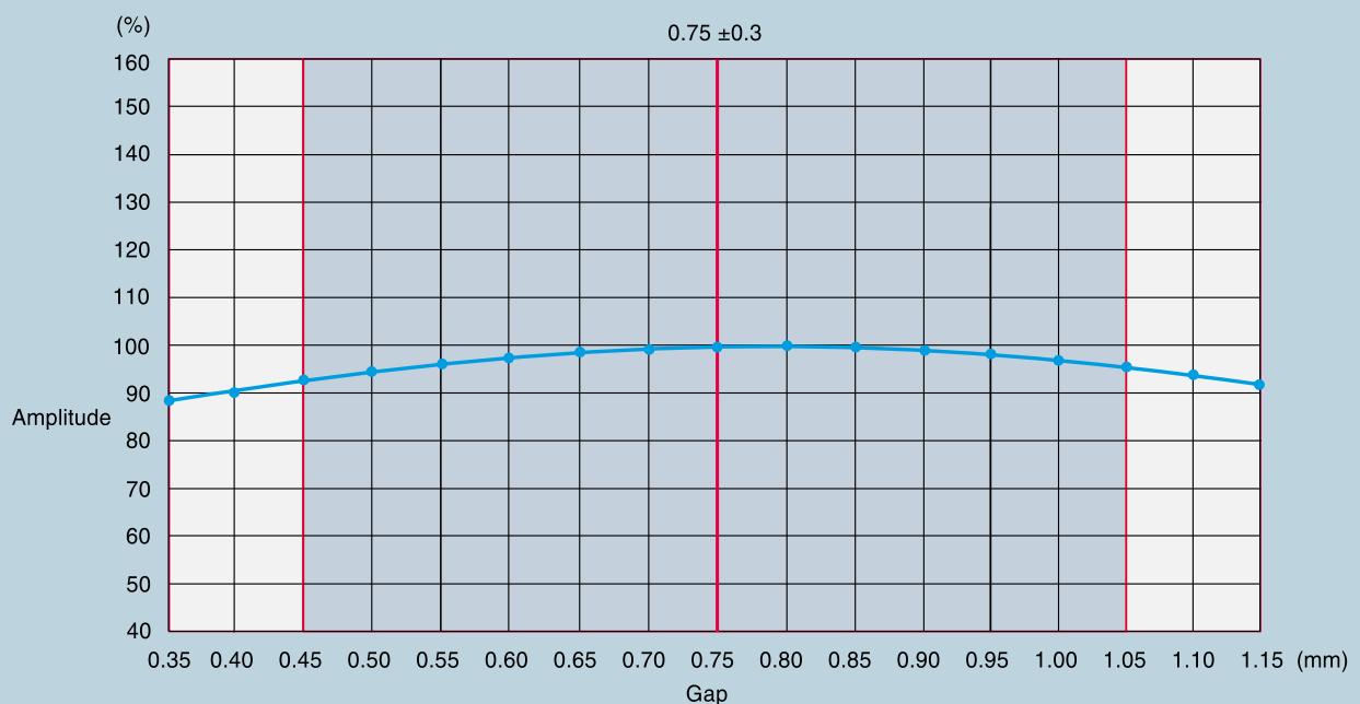
Reading head gap (mm) - vs. - Change in signal amplitude (%)
