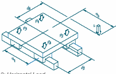
Figure 2: Horizontal Load
