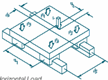
Figure 1: Horizontal Load
