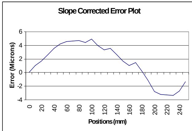
Slope Corrected Error Plot, Total error 8.5 microns
