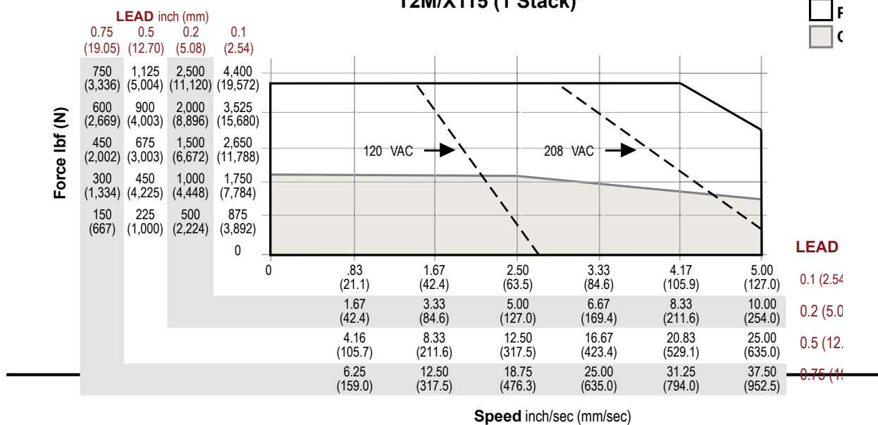
T2M/X115 (1 Stack)*
